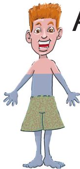
Surface Water
