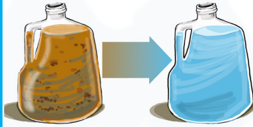
Runoff
