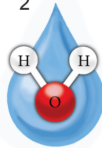
Evaporation
