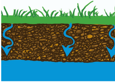
Major Pollutants
