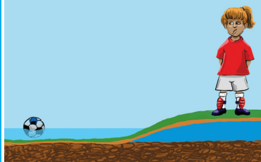
Drought
