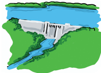
Reservoir
