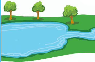
Surface Water
