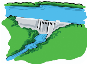
Reservoir
