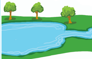
Surface Water
