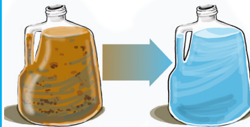
Aquifer
