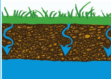
Infiltration
