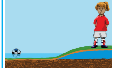
Subsidence
