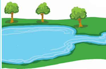
Surface Water
